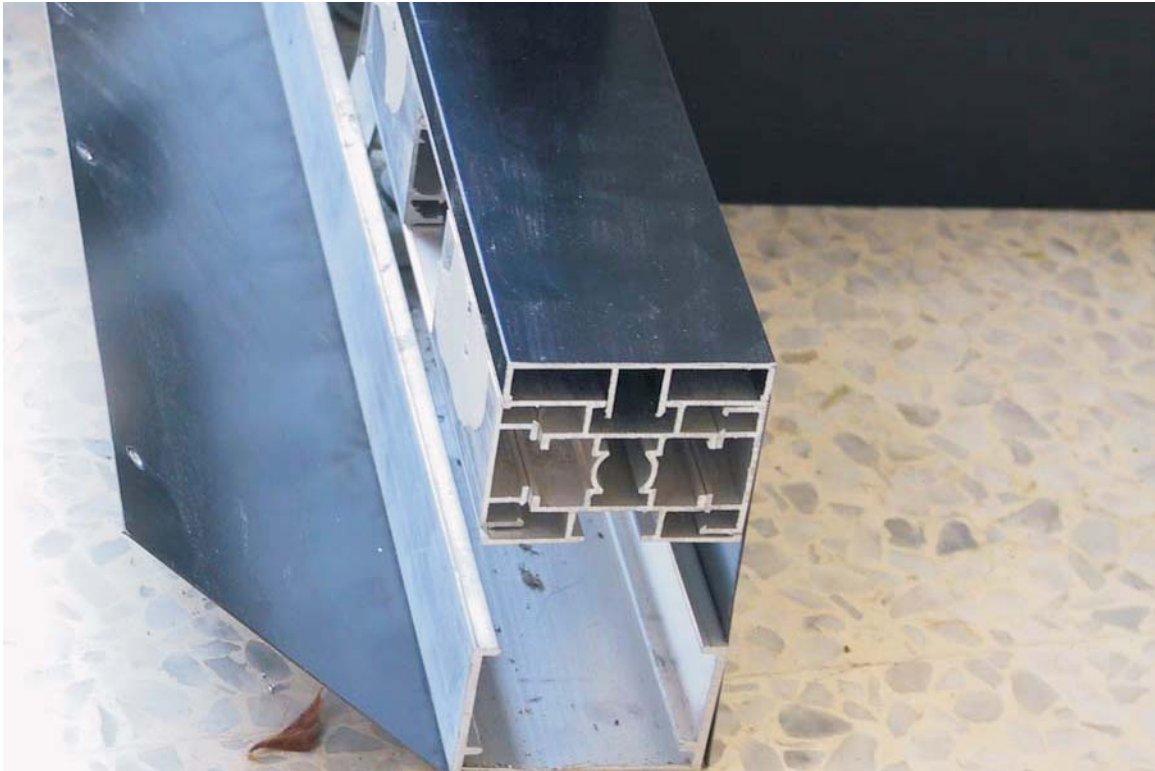
Skirting Installation
